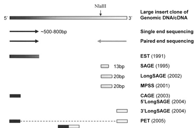
Figure 2. Sequencing-based methods for understanding genetic elements in genomes. The nucleotide information of DNA fragments can be spelled out by complete sequencing analysis. Alternatively, the large size of DNA fragments can be analyzed by single-end sequencing or paired-end sequencing. EST was the first tag-based approach, generating one tag per sequencing read, to represent full-length transcripts of expressed genes. The original SAGE tag extracts 13 bp next to the 3' most NlaIII site to tag the transcripts. LongSAGE and MPSS use MmeI as the tagging enzyme to generate 20-bp tags that can be specifically aligned to reference genome sequences. The CAGE and 5' LongSAGE tags are derived from the 5' end of cDNA fragments, and the 3' LongSAGE tags are derived from the 3' end of cDNA fragments. PET covalently combines the 5' and 3' signature tags of the same DNA fragment into one ditag unit.
